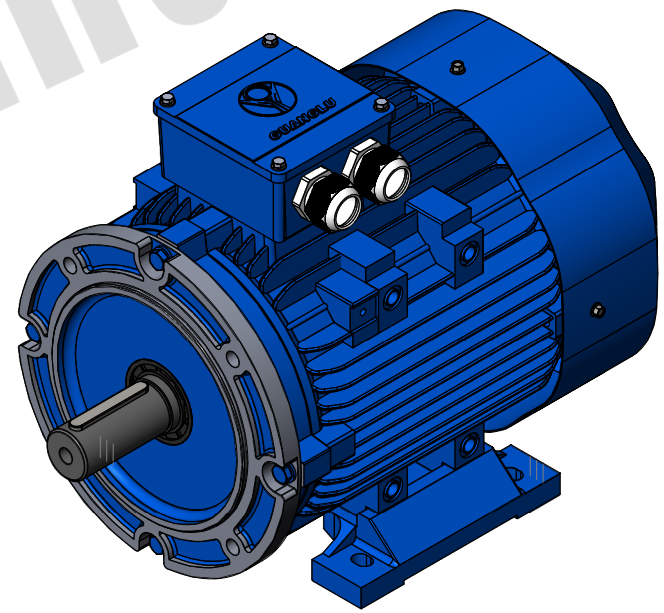
IE2-132S-B34B Mounting diagram
