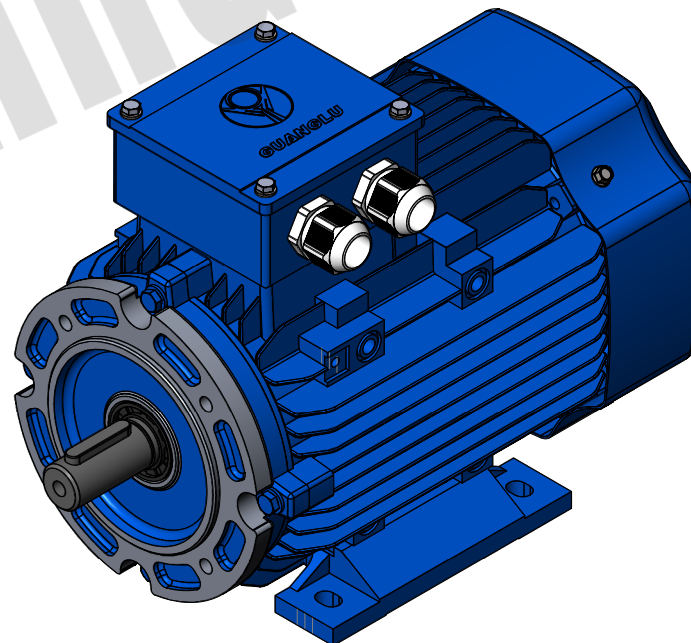
IE2-90L-B34B Mounting diagram
