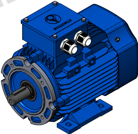
IE2-90S-B34B Mounting diagram
