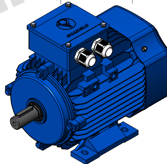
IE2-90S-B3 Mounting diagram
