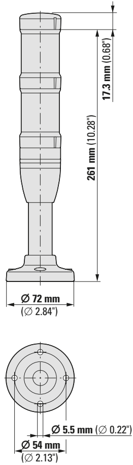
SL4-100-L-RG-24LED
